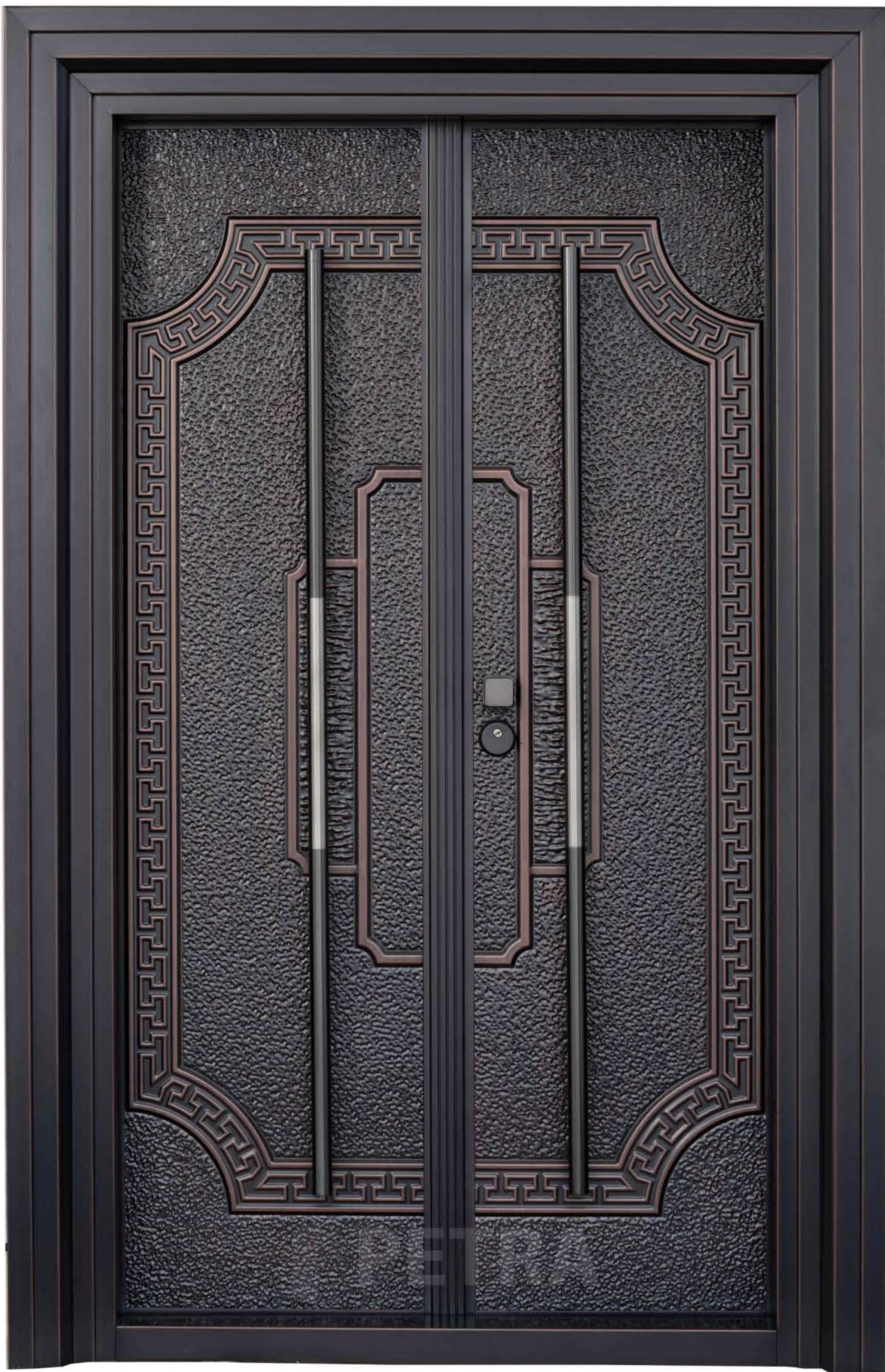
PTR 636 - 2050*1200*90MM 9" M\L (MOBH)
